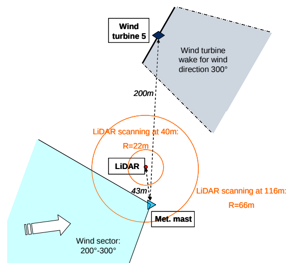
Figure 3: Measurement sector schematic
